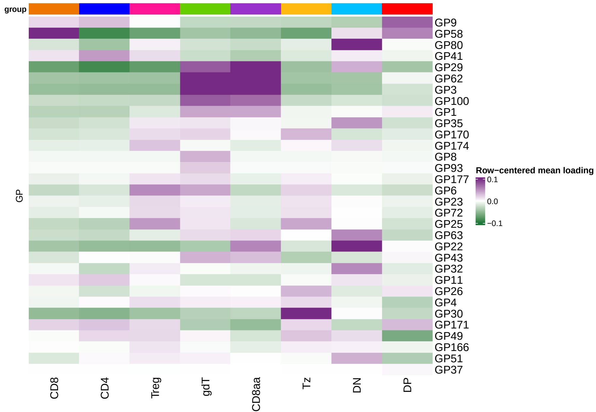
Row-centered GP mean loading: lineage (annotation_level1) the same 32 GPs, row order from (a)
